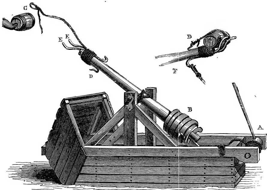
TRAPGET OR WAR-ENGINE, here drawn as used when casting Greek fire. A windlass. B weights of metal to pull down the beam. D catches. E fork holding the barrel. C catch which carries the rope that pulls down beam-head and is loosed when the Trapget goes off.
