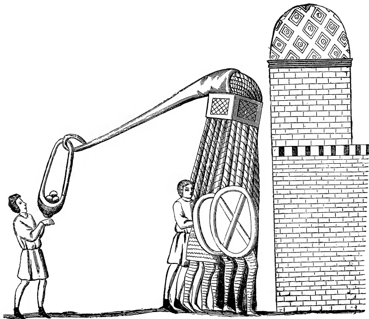
MACHINE FOR CASTING STONES. From a miniature of the Chevalier au Cygne MS. of the 13th century. Paris.
